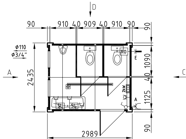
View A
